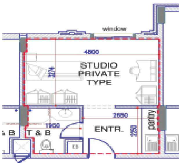
PRIVATE TYPE BEDROOM TOTAL AREA 26 M2
