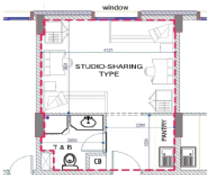
2-SHARING BEDROOM - TYPE 1 TOTAL AREA 26 M2
